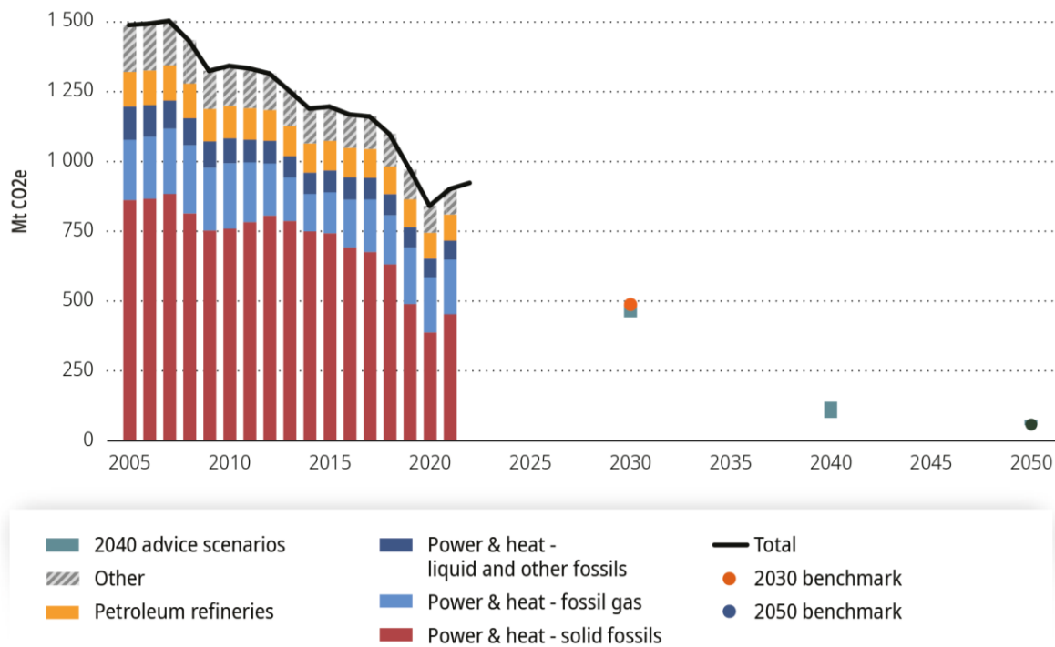
Figure 13 Indicator E1 – total GHG emissions of the energy supply sector
