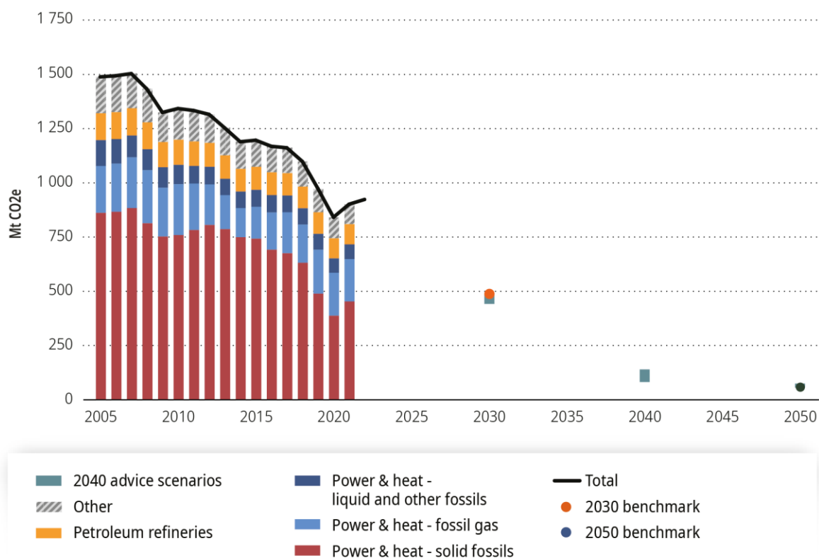
Figure 11 Indicator E1 – total GHG emission of the energy supply sector
